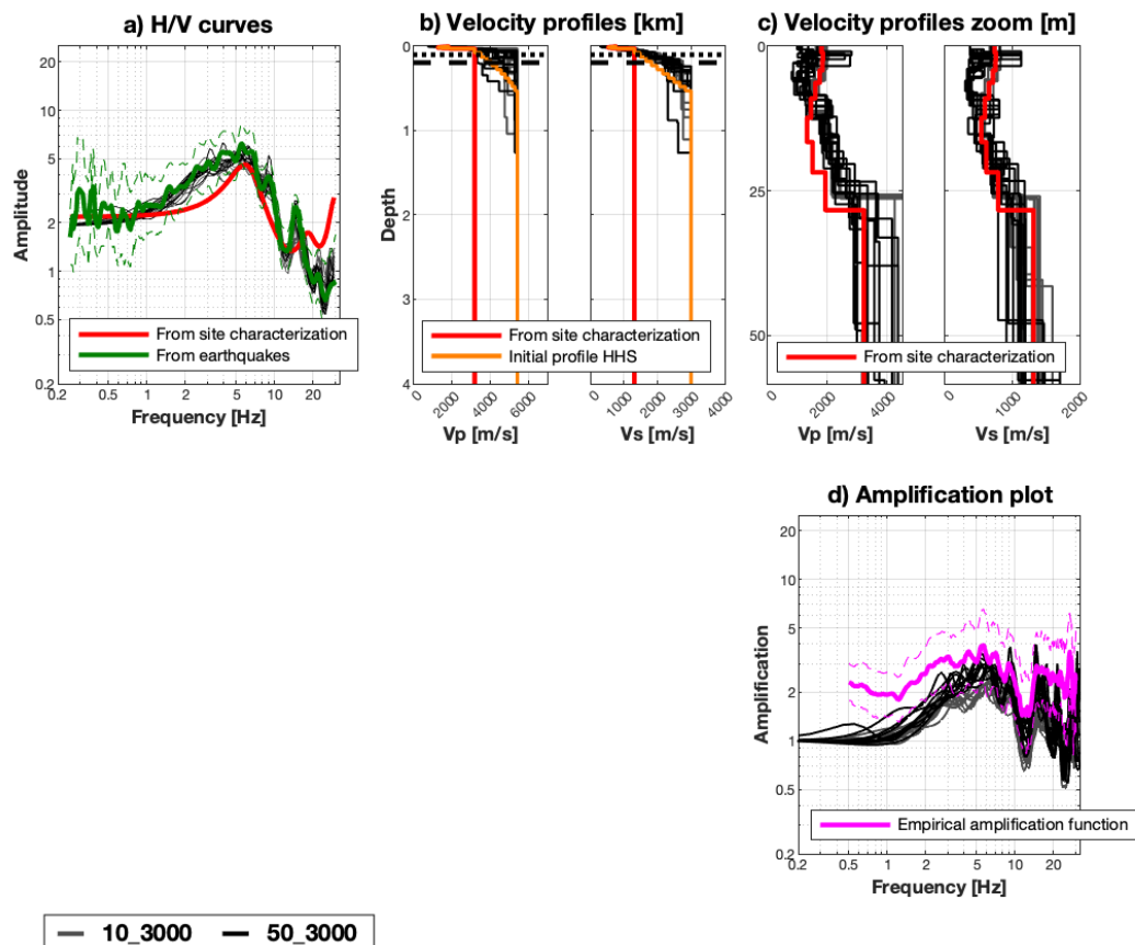
Figure 1: Estimated models from the HHS inversion for seismic station WEIN. The models estimated by the HHS algorithm are shown in dark gray and black. In the velocity profiles plots (b), the dotted and dashed horizontal lines correspond to the QWL depth at a frequency of 0.5 \cdot f_0 ( = 2.65 Hz) and to 2 times the QWL depth, respectively.
