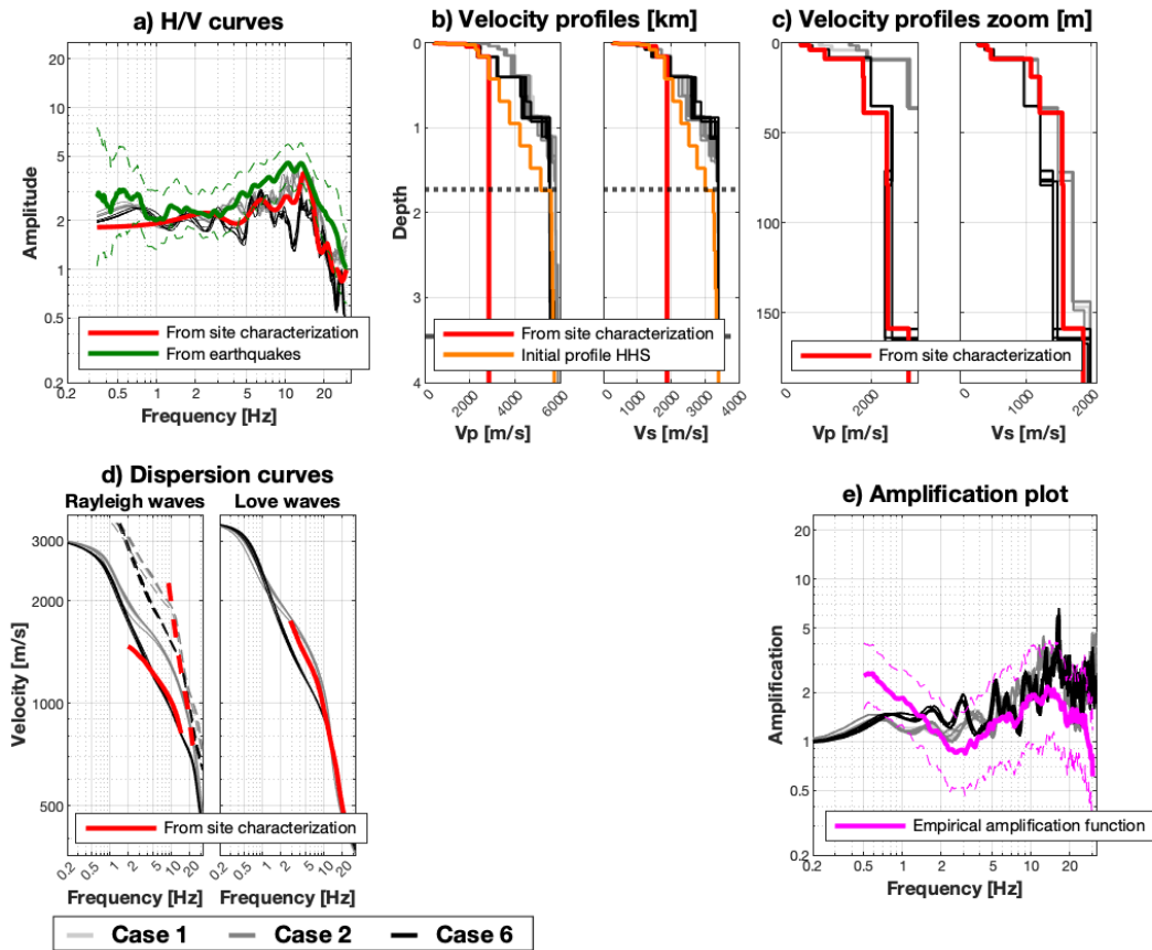
Figure 2: Estimated models from the HHS inversion for seismic station WALHA. The models estimated by the HHS algorithm are shown in light/dark gray and black. In the velocity profiles plots (b), the dotted and dashed horizontal lines correspond to the QWL depth at a frequency of 0.5 \cdot f_0 ( = 0.37 Hz) and to 2 times the QWL depth, respectively.
