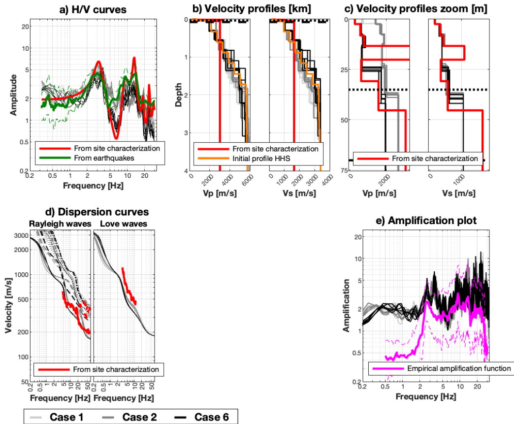
Figure 2: Estimated models from the HHS inversion for seismic station SZEK. The models estimated by the HHS algorithm are shown in light/dark gray and black. In the velocity profiles plots (b), the dotted and dashed horizontal lines correspond to the QWL depth at a frequency of 0.5 \cdot f_0 ( = 0.49 Hz) and to 2 times the QWL depth, respectively.
