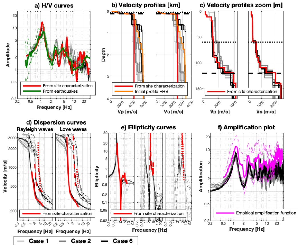
Figure 2: Estimated models from the HHS inversion for seismic station SYVP. The models estimated by the HHS algorithm are shown in light/dark gray and black. In the velocity profiles plots (b), the dotted and dashed horizontal lines correspond to the QWL depth at a frequency of 0.5 \cdot f_0 ( = 0.58 Hz) and to 2 times the QWL depth, respectively.
