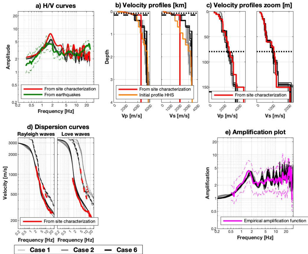
Figure 2: Estimated models from the HHS inversion for seismic station SVEJ. The models estimated by the HHS algorithm are shown in light/dark gray and black. In the velocity profiles plots (b), the dotted and dashed horizontal lines correspond to the QWL depth at a frequency of 0.5 \cdot f_0 ( = 0.94 Hz) and to 2 times the QWL depth, respectively.
