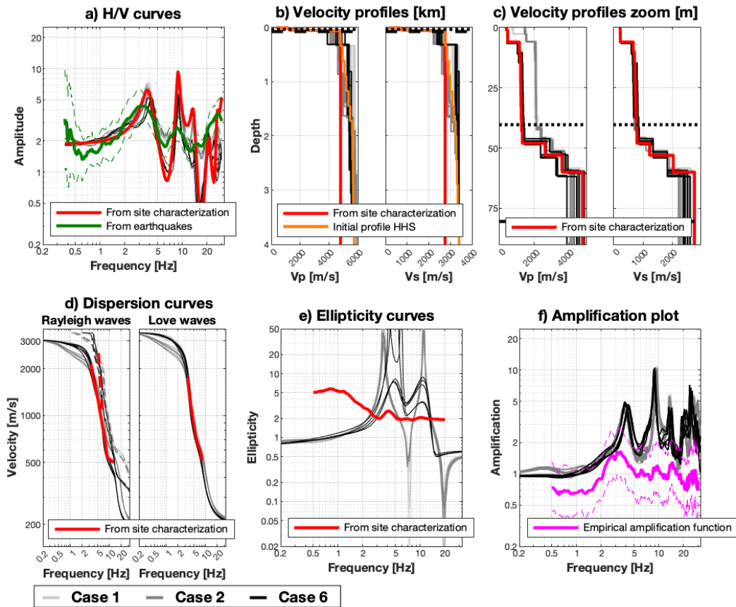
Figure 2: Estimated models from the HHS inversion for seismic station SVAM. The models estimated by the HHS algorithm are shown in light/dark gray and black. In the velocity profiles plots (b), the dotted and dashed horizontal lines correspond to the QWL depth at a frequency of 0.5 \cdot f_0 ( = 1.93 Hz) and to 2 times the QWL depth, respectively.
