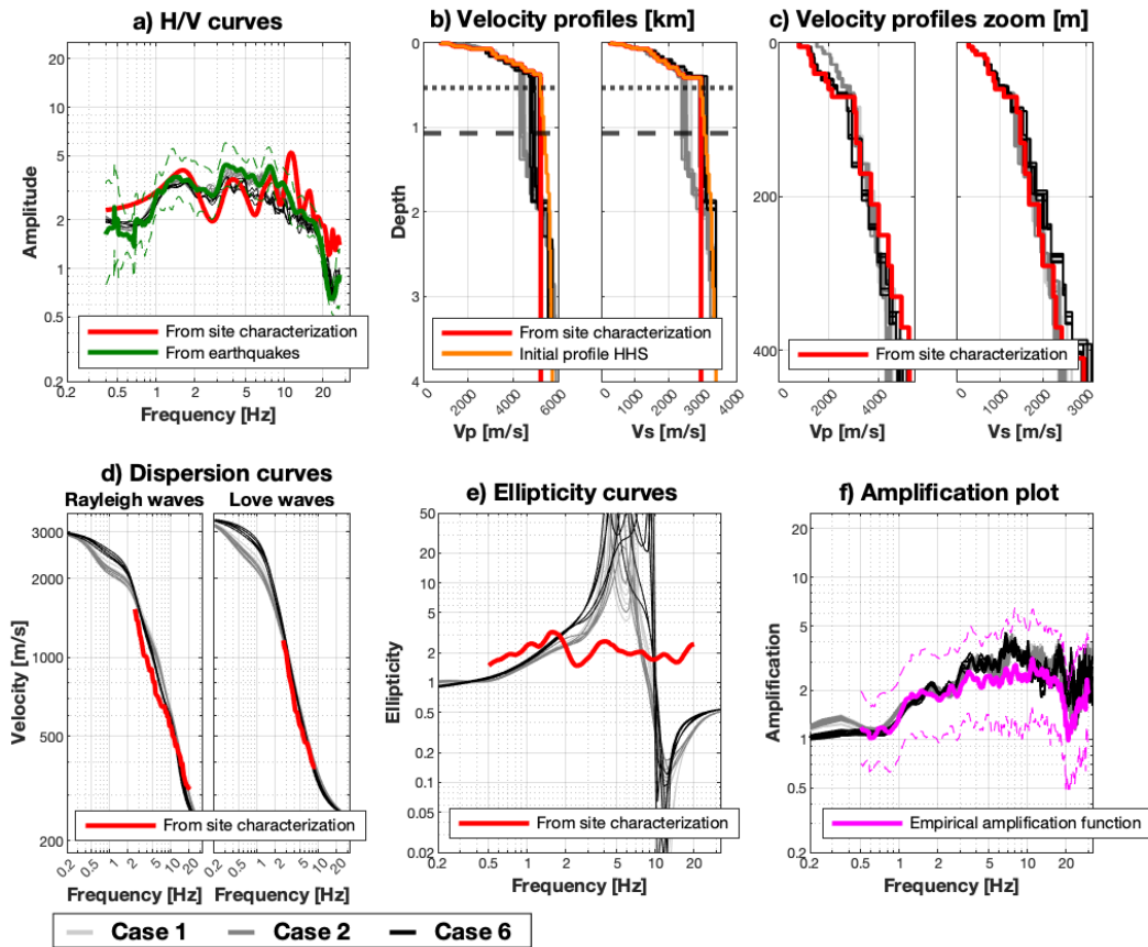
Figure 2: Estimated models from the HHS inversion for seismic station STRW. The models estimated by the HHS algorithm are shown in light/dark gray and black. In the velocity profiles plots (b), the dotted and dashed horizontal lines correspond to the QWL depth at a frequency of 0.5 \cdot f_0 ( = 0.74 Hz) and to 2 times the QWL depth, respectively.
