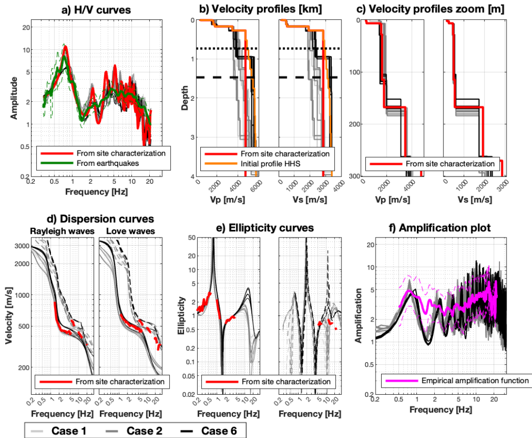
Figure 2: Estimated models from the HHS inversion for seismic station STHK. The models estimated by the HHS algorithm are shown in light/dark gray and black. In the velocity profiles plots (b), the dotted and dashed horizontal lines correspond to the QWL depth at a frequency of 0.5 \cdot f_0 ( = 0.41 Hz) and to 2 times the QWL depth, respectively.
