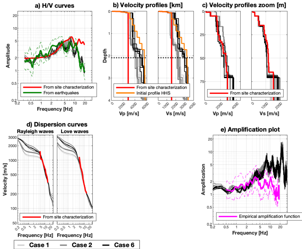
Figure 2: Estimated models from the HHS inversion for seismic station STGK. The models estimated by the HHS algorithm are shown in light/dark gray and black. In the velocity profiles plots (b), the dotted horizontal line corresponds to the QWL depth at a frequency of 0.5 \cdot f_0 ( = 0.22 Hz).
