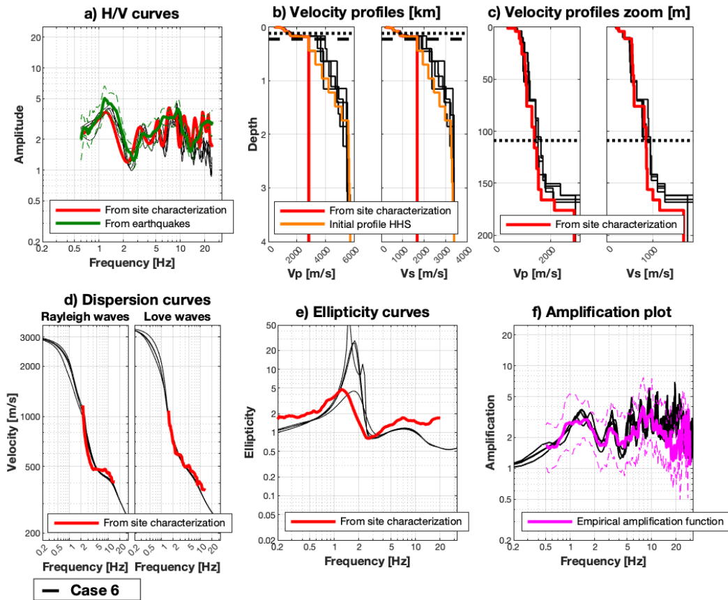
Figure 2: Estimated models from the HHS inversion for seismic station SOLZ. The models estimated by the HHS algorithm are shown in black. In the velocity profiles plots (b), the dotted and dashed horizontal lines correspond to the QWL depth at a frequency of 0.5 \cdot f_0 ( = 0.34 Hz) and to 2 times the QWL depth, respectively.
