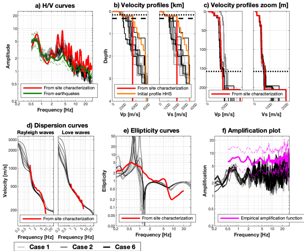
Figure 2: Estimated models from the HHS inversion for seismic station SOLB. The models estimated by the HHS algorithm are shown in light/dark gray and black. In the velocity profiles plots (b), the dotted and dashed horizontal lines correspond to the QWL depth at a frequency of 0.5 \cdot f_0 ( = 0.34 Hz) and to 2 times the QWL depth, respectively.
