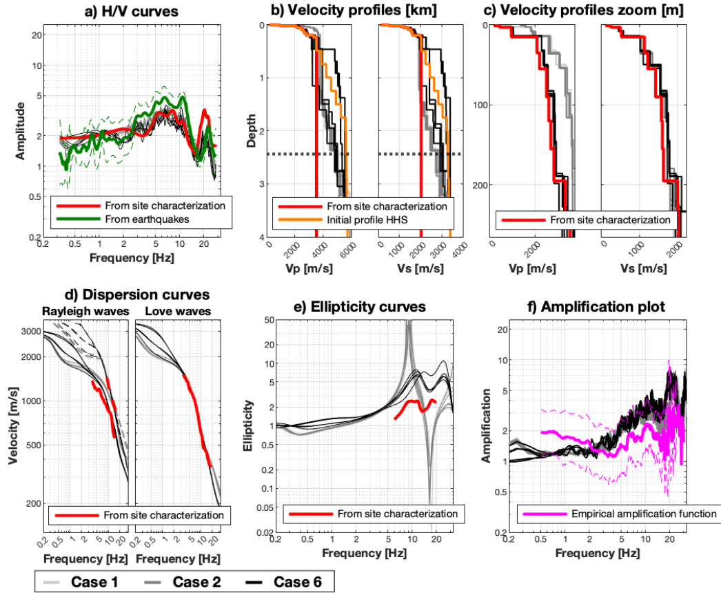
Figure 2: Estimated models from the HHS inversion for seismic station SMOE. The models estimated by the HHS algorithm are shown in light/dark gray and black. In the velocity profiles plots (b), the dotted and dashed horizontal lines correspond to the QWL depth at a frequency of 0.5 \cdot f_0 ( = 0.24 Hz) and to 2 times the QWL depth, respectively.
