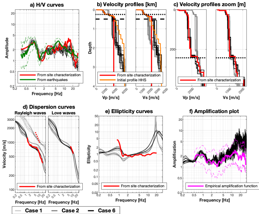
Figure 2: Estimated models from the HHS inversion for seismic station SMAO. The models estimated by the HHS algorithm are shown in light/dark gray and black. In the velocity profiles plots (b), the dotted and dashed horizontal lines correspond to the QWL depth at a frequency of 0.5 \cdot f_0 ( = 0.39 Hz) and to 2 times the QWL depth, respectively.
