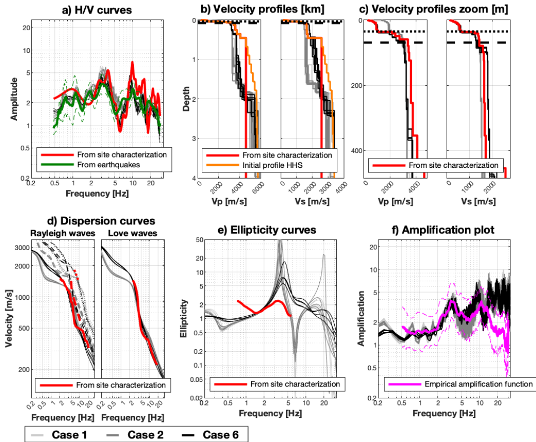
Figure 2: Estimated models from the HHS inversion for seismic station SLCF. The models estimated by the HHS algorithm are shown in light/dark gray and black. In the velocity profiles plots (b), the dotted and dashed horizontal lines correspond to the QWL depth at a frequency of 0.5 \cdot f_0 ( = 0.4 Hz) and to 2 times the QWL depth, respectively.
