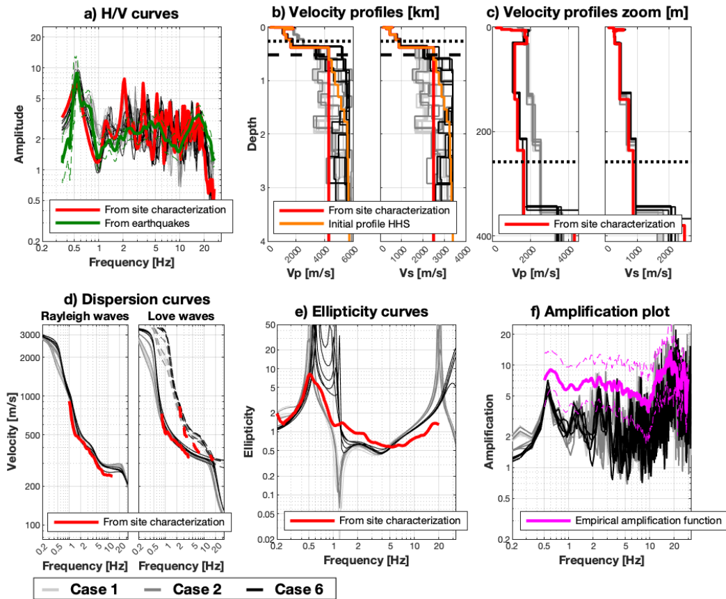
Figure 2: Estimated models from the HHS inversion for seismic station SINS. The models estimated by the HHS algorithm are shown in light/dark gray and black. In the velocity profiles plots (b), the dotted and dashed horizontal lines correspond to the QWL depth at a frequency of 0.5 \cdot f_0 ( = 0.3 Hz) and to 2 times the QWL depth, respectively.
