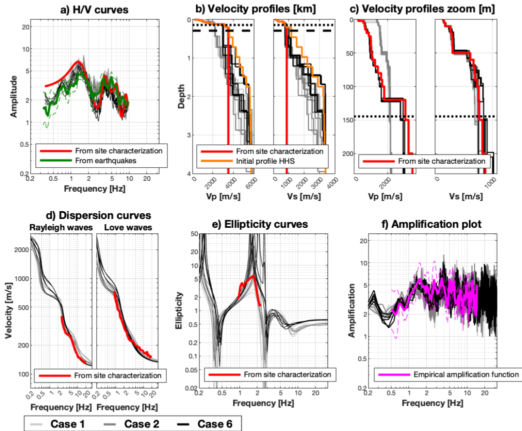
Figure 2: Estimated models from the HHS inversion for seismic station SHEK. The models estimated by the HHS algorithm are shown in light/dark gray and black. In the velocity profiles plots (b), the dotted and dashed horizontal lines correspond to the QWL depth at a frequency of 0.5 \cdot f_0 ( = 0.75 Hz) and to 2 times the QWL depth, respectively.
