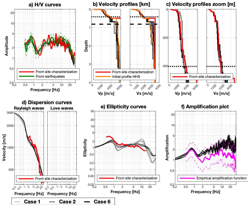
Figure 2: Estimated models from the HHS inversion for seismic station SGRA. The models estimated by the HHS algorithm are shown in light/dark gray and black. In the velocity profiles plots (b), the dotted and dashed horizontal lines correspond to the QWL depth at a frequency of 0.5 \cdot f_0 ( = 0.4 Hz) and to 2 times the QWL depth, respectively.
