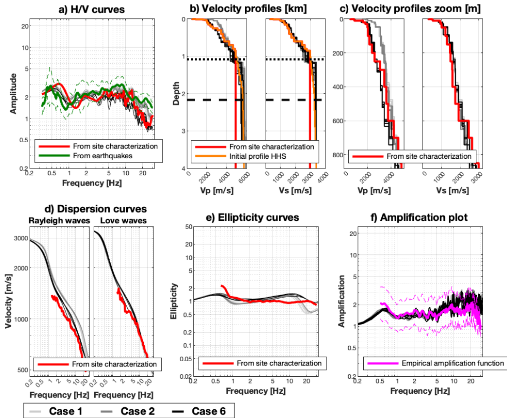
Figure 2: Estimated models from the HHS inversion for seismic station SCUG. The models estimated by the HHS algorithm are shown in light/dark gray and black. In the velocity profiles plots (b), the dotted and dashed horizontal lines correspond to the QWL depth at a frequency of 0.5 \cdot f_0 ( = 0.26 Hz) and to 2 times the QWL depth, respectively.
