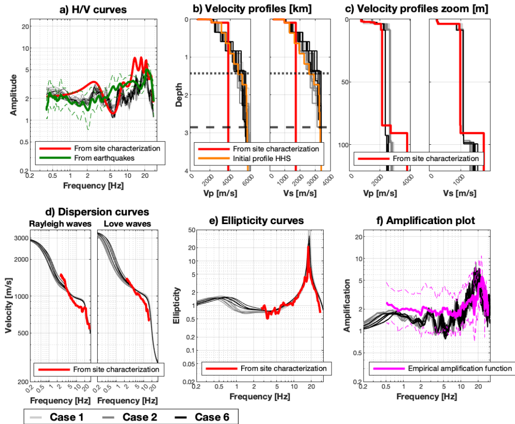
Figure 2: Estimated models from the HHS inversion for seismic station SBUL. The models estimated by the HHS algorithm are shown in light/dark gray and black. In the velocity profiles plots (b), the dotted and dashed horizontal lines correspond to the QWL depth at a frequency of 0.5 \cdot f_0 ( = 0.35 Hz) and to 2 times the QWL depth, respectively.
