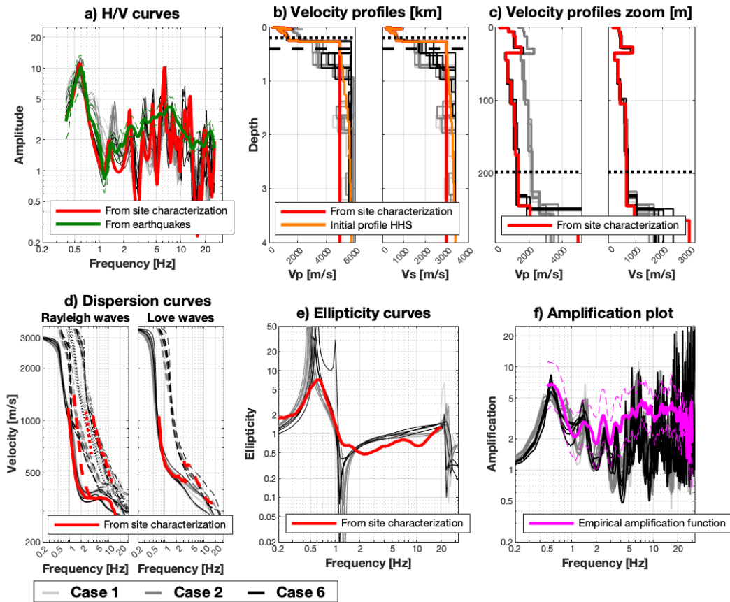
Figure 2: Estimated models from the HHS inversion for seismic station SBUH. The models estimated by the HHS algorithm are shown in light/dark gray and black. In the velocity profiles plots (b), the dotted and dashed horizontal lines correspond to the QWL depth at a frequency of 0.5 \cdot f_0 ( = 0.29 Hz) and to 2 times the QWL depth, respectively.
