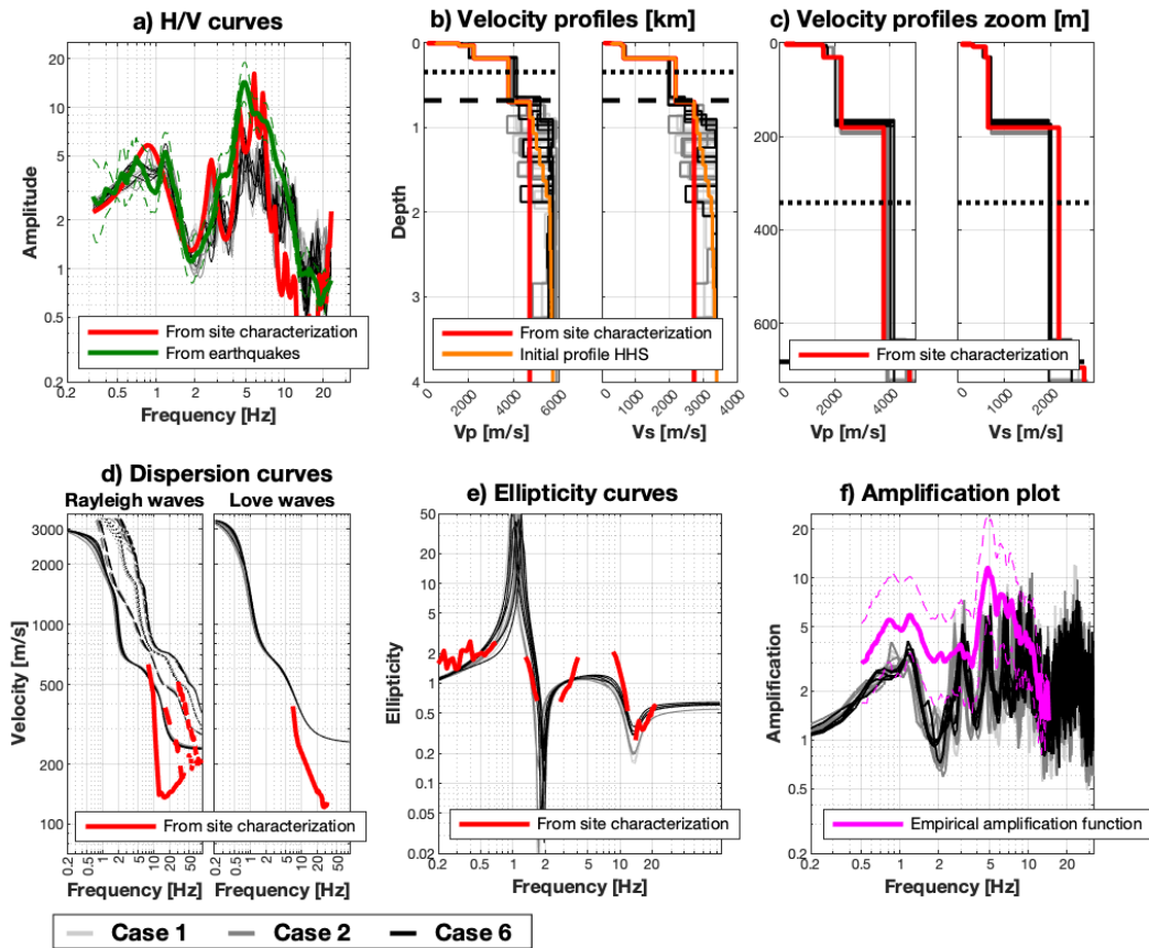
Figure 2: Estimated models from the HHS inversion for seismic station SBIK. The models estimated by the HHS algorithm are shown in light/dark gray and black. In the velocity profiles plots (b), the dotted and dashed horizontal lines correspond to the QWL depth at a frequency of 0.5 \cdot f_0 ( = 0.34 Hz) and to 2 times the QWL depth, respectively.
