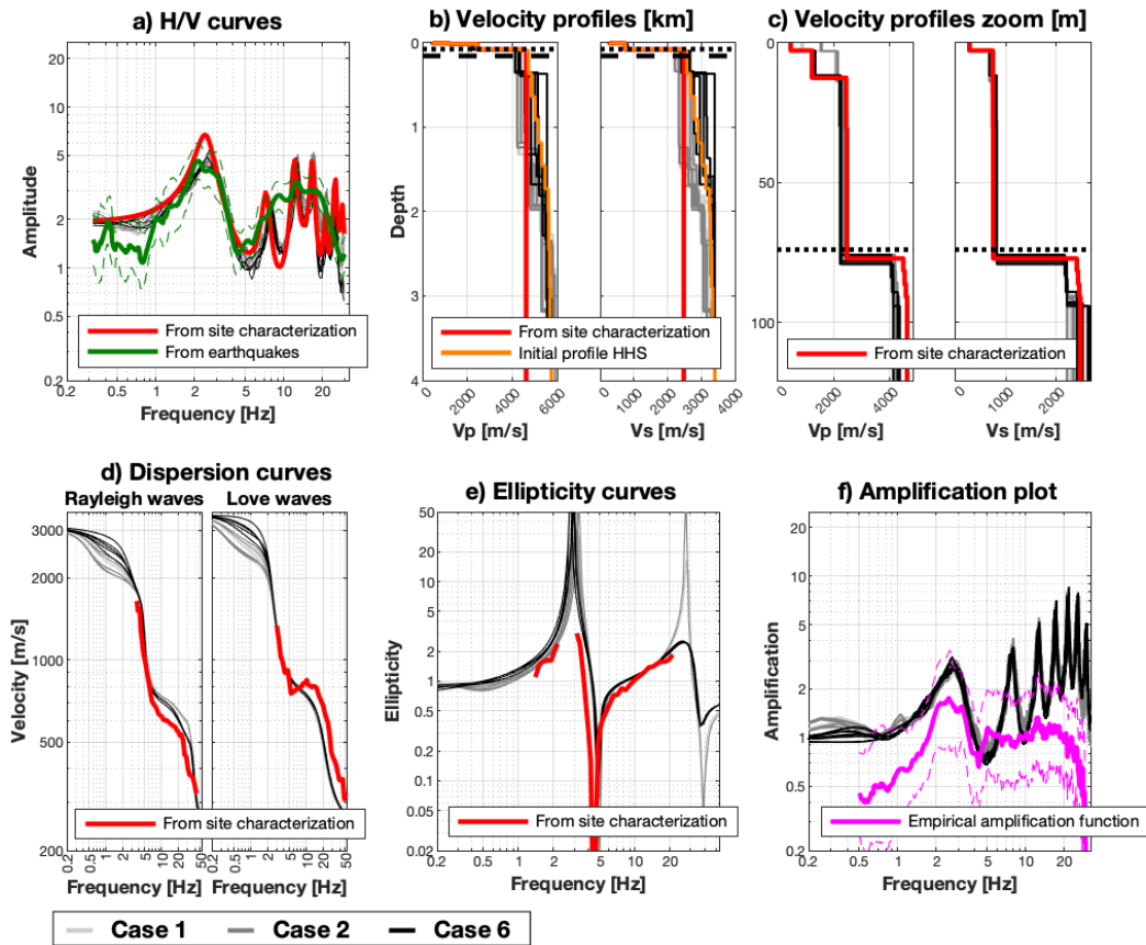
Figure 2: Estimated models from the HHS inversion for seismic station SBGN. The models estimated by the HHS algorithm are shown in light/dark gray and black. In the velocity profiles plots (b), the dotted and dashed horizontal lines correspond to the QWL depth at a frequency of 0.5 \cdot f_0 ( = 0.52 Hz) and to 2 times the QWL depth, respectively.
