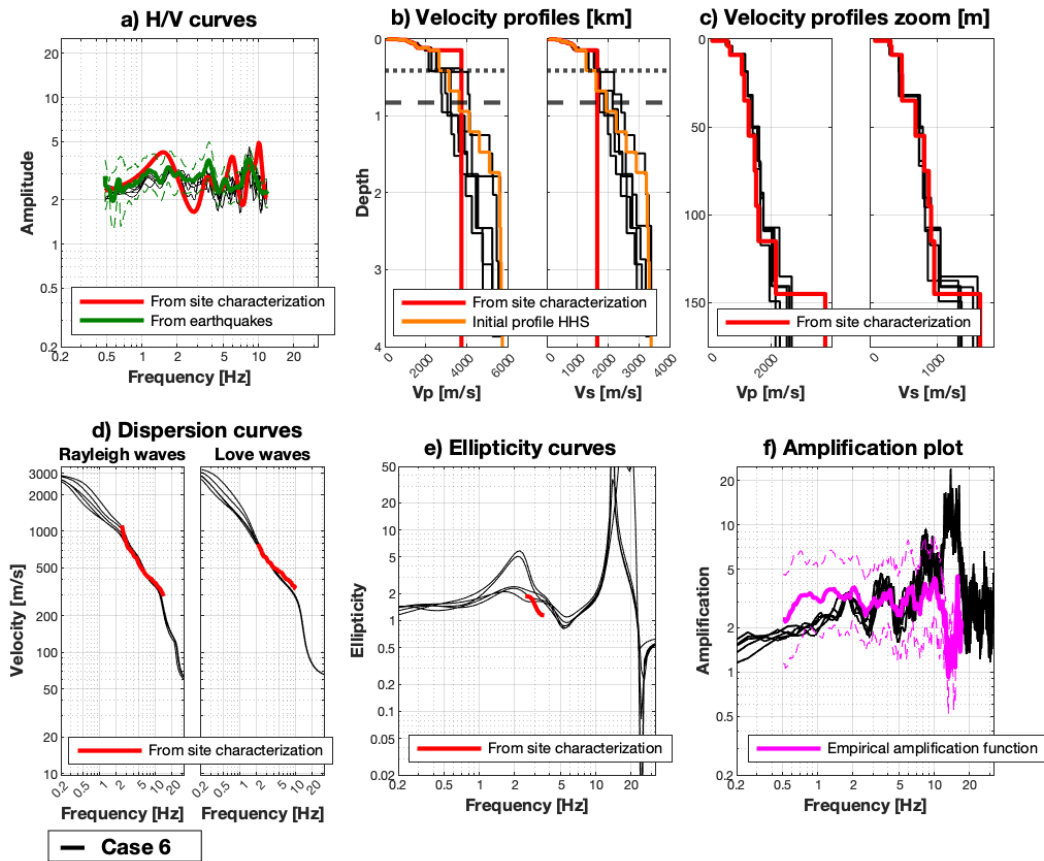
Figure 2: Estimated models from the HHS inversion for seismic station SBERN. The models estimated by the HHS algorithm are shown in black. In the velocity profiles plots (b), the dotted and dashed horizontal lines correspond to the QWL depth at a frequency of 0.5 \cdot f_0 ( = 0.57 Hz) and to 2 times the QWL depth, respectively.
