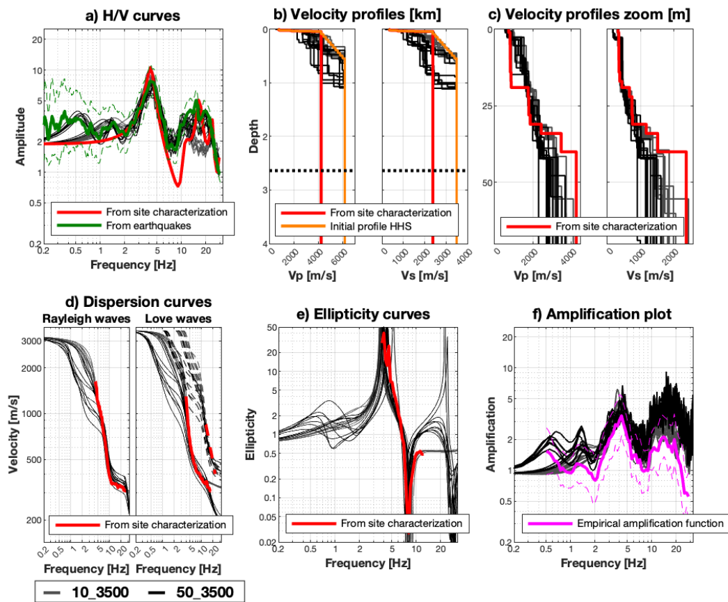
Figure 1: Estimated models from the HHS inversion for seismic station SBEG. The models estimated by the HHS algorithm are shown in dark gray and black. In the velocity profiles plots (b), the dotted and dashed horizontal lines correspond to the QWL depth at a frequency of 0.5 \cdot f_0 ( = 0.27 Hz) and to 2 times the QWL depth, respectively.
