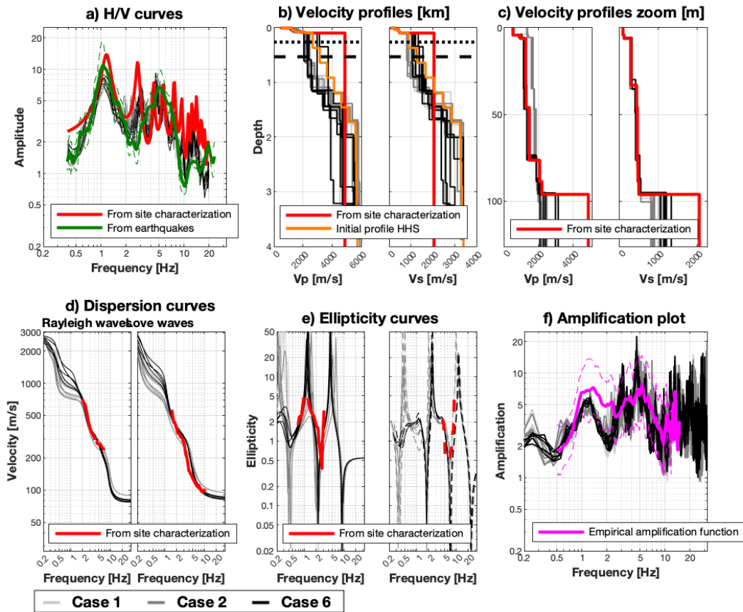
Figure 2: Estimated models from the HHS inversion for seismic station SBAS. The models estimated by the HHS algorithm are shown in light/dark gray and black. In the velocity profiles plots (b), the dotted and dashed horizontal lines correspond to the QWL depth at a frequency of 0.5 \cdot f_0 ( = 0.55 Hz) and to 2 times the QWL depth, respectively.
