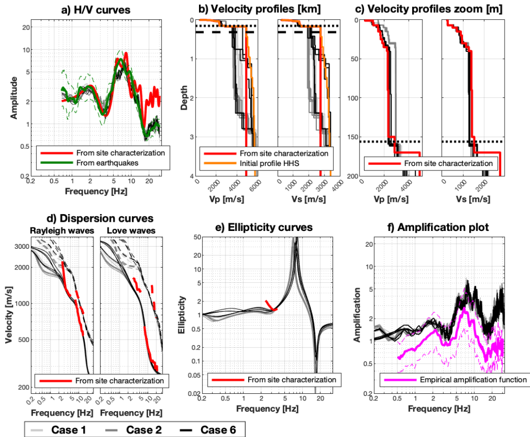
Figure 2: Estimated models from the HHS inversion for seismic station SARK. The models estimated by the HHS algorithm are shown in light/dark gray and black. In the velocity profiles plots (b), the dotted and dashed horizontal lines correspond to the QWL depth at a frequency of 0.5 \cdot f_0 ( = 0.9 Hz) and to 2 times the QWL depth, respectively.
