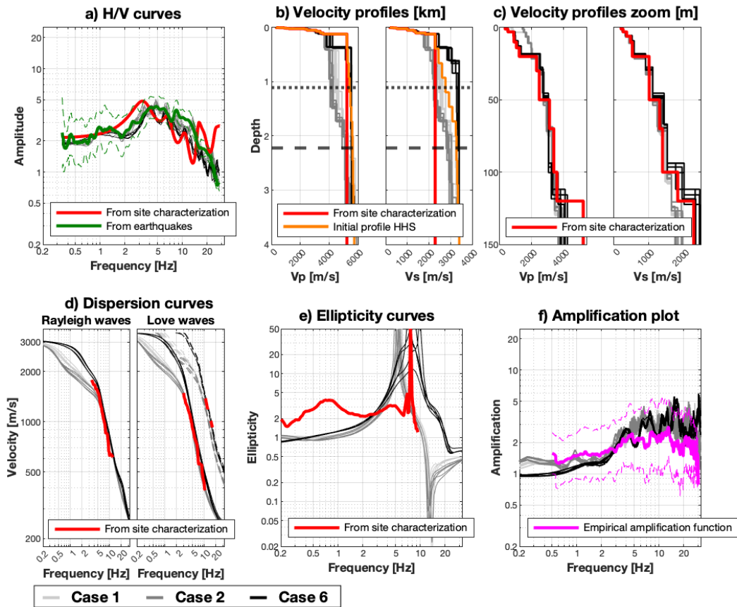
Figure 2: Estimated models from the HHS inversion for seismic station SAPK. The models estimated by the HHS algorithm are shown in light/dark gray and black. In the velocity profiles plots (b), the dotted and dashed horizontal lines correspond to the QWL depth at a frequency of 0.5 \cdot f_0 ( = 0.5 Hz) and to 2 times the QWL depth, respectively.
