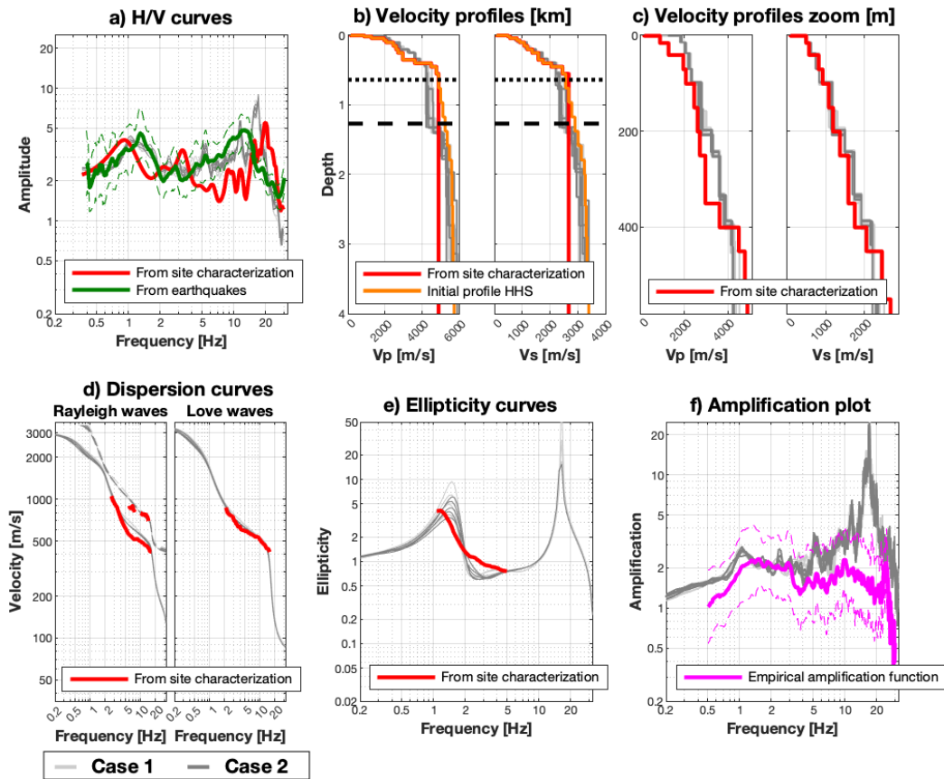
Figure 2: Estimated models from the HHS inversion for seismic station SALTS. The models estimated by the HHS algorithm are shown in light and dark gray. In the velocity profiles plots (b), the dotted and dashed horizontal lines correspond to the QWL depth at a frequency of 0.5 \cdot f_0 ( = 0.55 Hz) and to 2 times the QWL depth, respectively.
