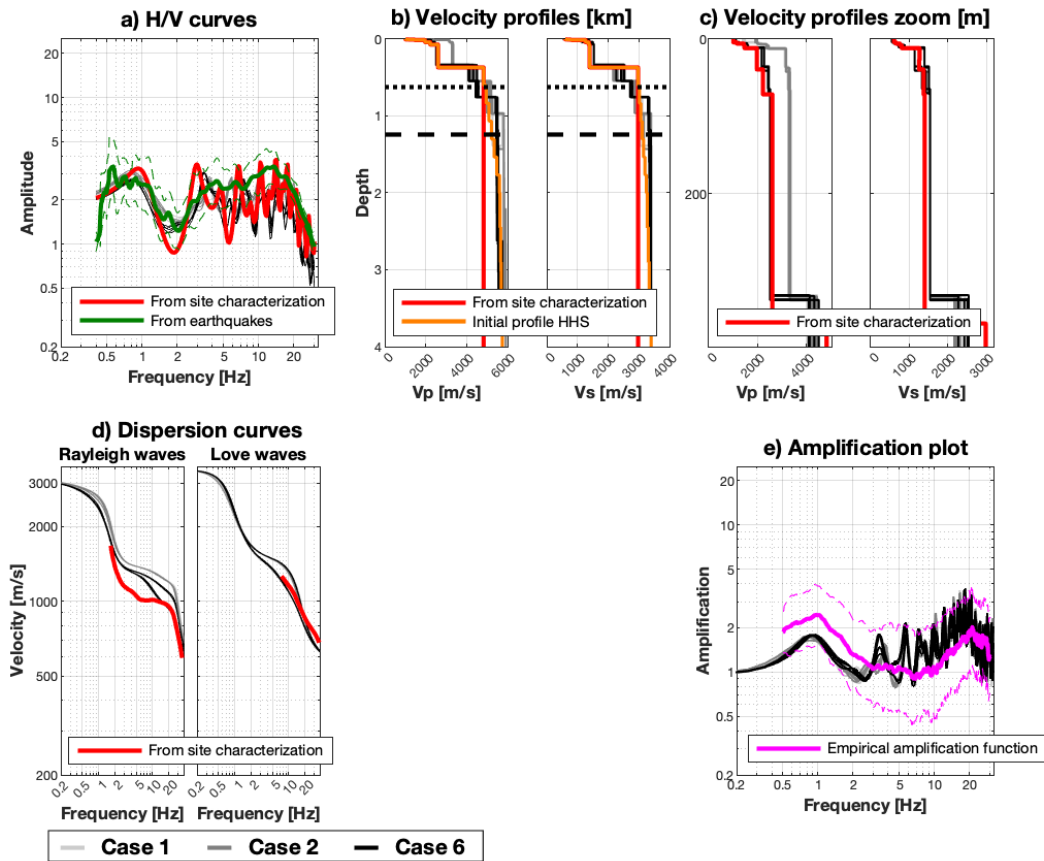
Figure 2: Estimated models from the HHS inversion for seismic station ROTHE. The models estimated by the HHS algorithm are shown in light/dark gray and black. In the velocity profiles plots (b), the dotted and dashed horizontal lines correspond to the QWL depth at a frequency of 0.5 \cdot f_0 ( = 0.4 Hz) and to 2 times the QWL depth, respectively.
