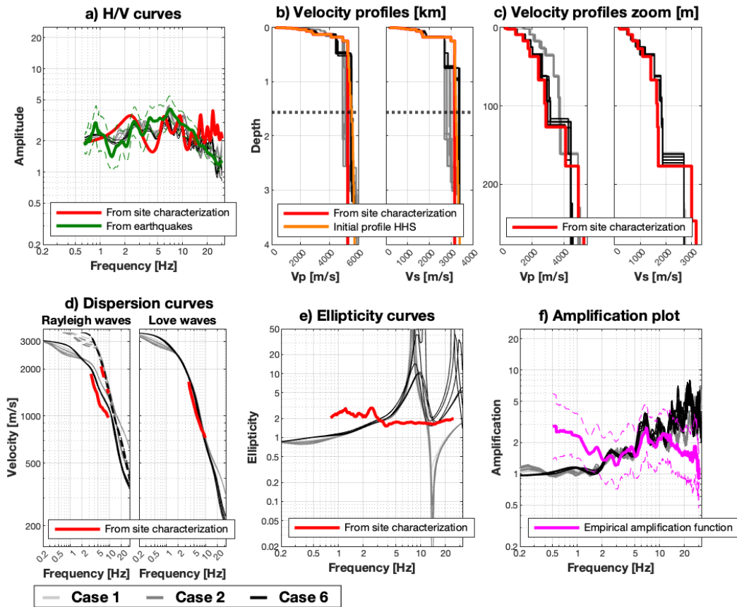
Figure 2: Estimated models from the HHS inversion for seismic station MTI03. The models estimated by the HHS algorithm are shown in light/dark gray and black. In the velocity profiles plots (b), the dotted and dashed horizontal lines correspond to the QWL depth at a frequency of 0.5 \cdot f_0 ( = 0.43 Hz) and to 2 times the QWL depth, respectively.
