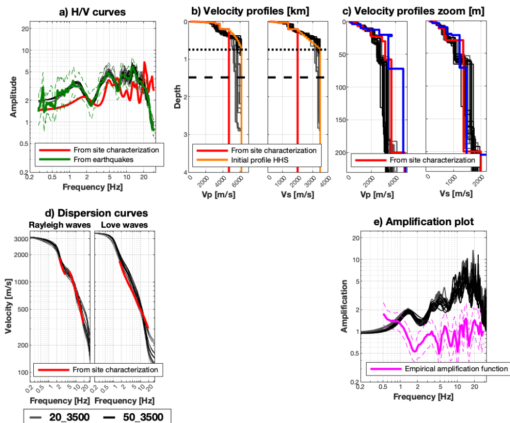
Figure 1: Estimated models from the HHS inversion for seismic station HAMIK. The models estimated by the HHS algorithm are shown in dark gray and black. In the velocity profiles plots (b), the dotted and dashed horizontal lines correspond to the QWL depth at a frequency of 0.5 \cdot f_0 ( = 0.67 Hz) and to 2 times the QWL depth, respectively. The velocity profile in blue is the MAP model from Neopsy (Hallo et al., 2021)
