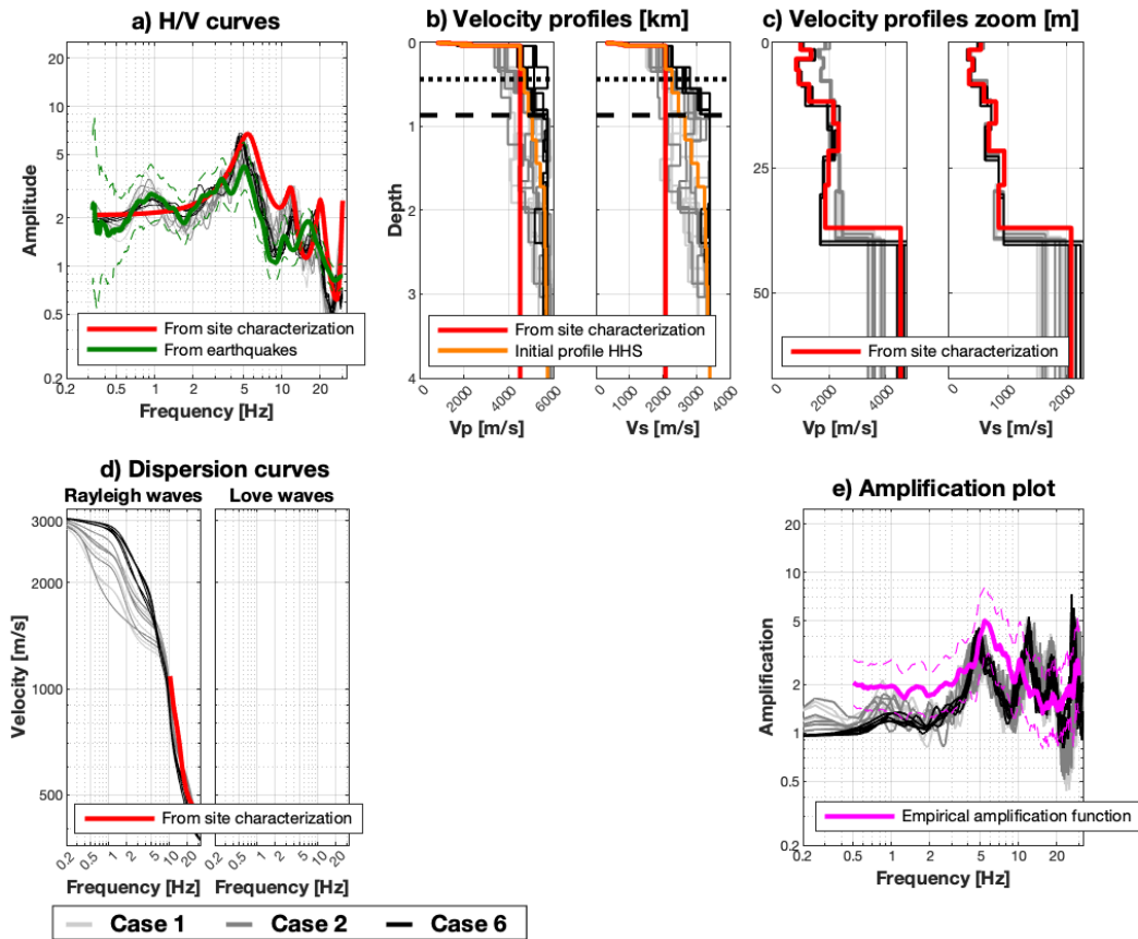
Figure 2: Estimated models from the HHS inversion for seismic station FLACH. The models estimated by the HHS algorithm are shown in light/dark gray and black. In the velocity profiles plots (b), the dotted and dashed horizontal lines correspond to the QWL depth at a frequency of 0.5 \cdot f_0 ( = 0.46 Hz) and to 2 times the QWL depth, respectively.
