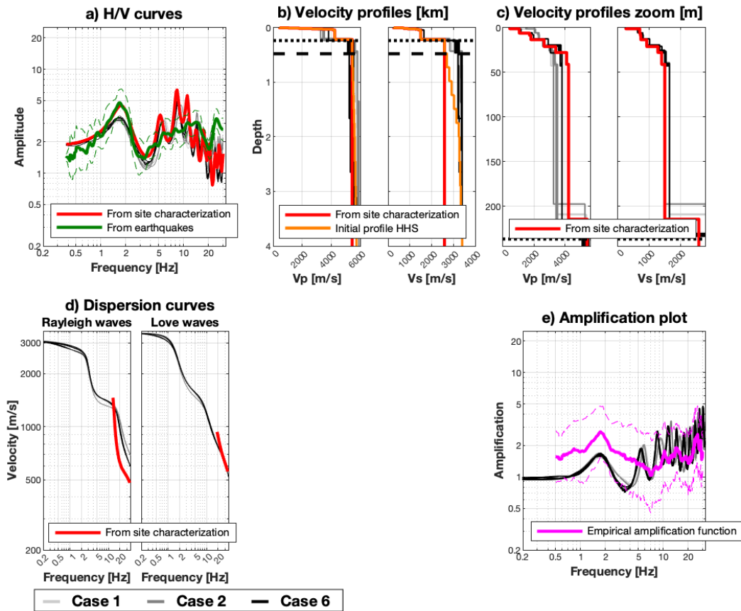
Figure 2: Estimated models from the HHS inversion for seismic station EMMET. The models estimated by the HHS algorithm are shown in light/dark gray and black. In the velocity profiles plots (b), the dotted and dashed horizontal lines correspond to the QWL depth at a frequency of 0.5 \cdot f_0 ( = 0.87 Hz) and to 2 times the QWL depth, respectively.
