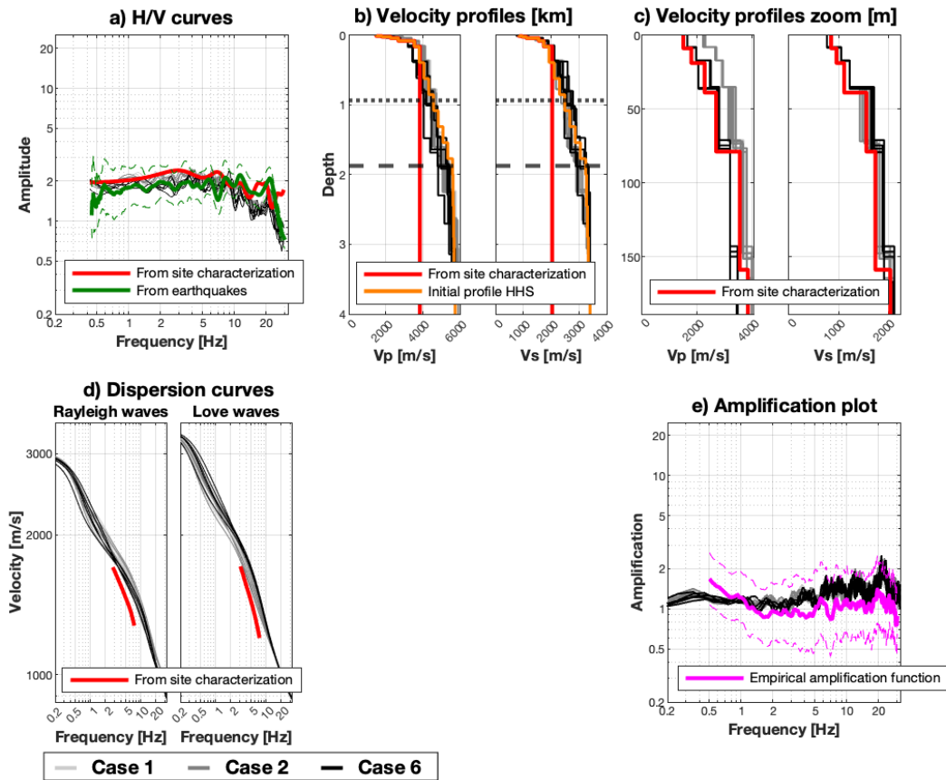
Figure 2: Estimated models from the HHS inversion for seismic station DAGMA. The models estimated by the HHS algorithm are shown in light/dark gray and black. In the velocity profiles plots (b), the dotted and dashed horizontal lines correspond to the QWL depth at a frequency of 0.5 \cdot f_0 ( = 0.59 Hz) and to 2 times the QWL depth, respectively.
