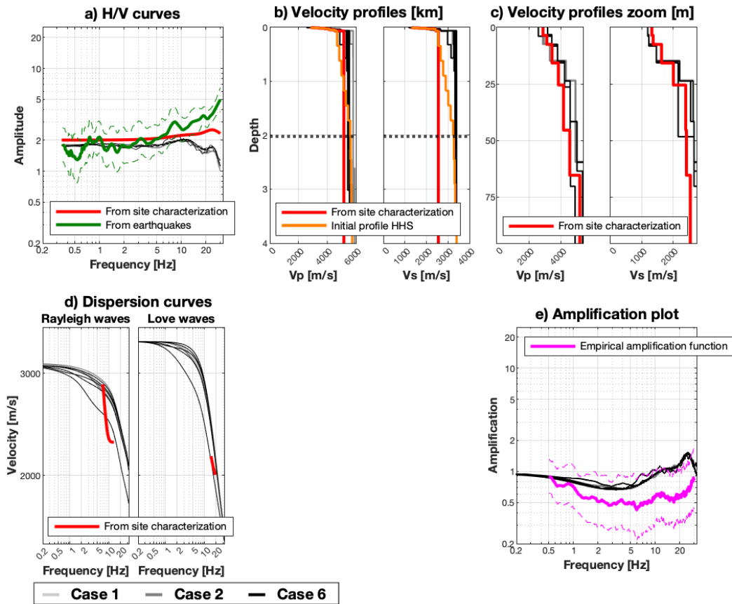
Figure 2: Estimated models from the HHS inversion for seismic station BERGE. The models estimated by the HHS algorithm are shown in light/dark gray and black. In the velocity profiles plots (b), the dotted and dashed horizontal lines correspond to the QWL depth at a frequency of 0.5 \cdot f_0 ( = 0.43 Hz) and to 2 times the QWL depth, respectively.
