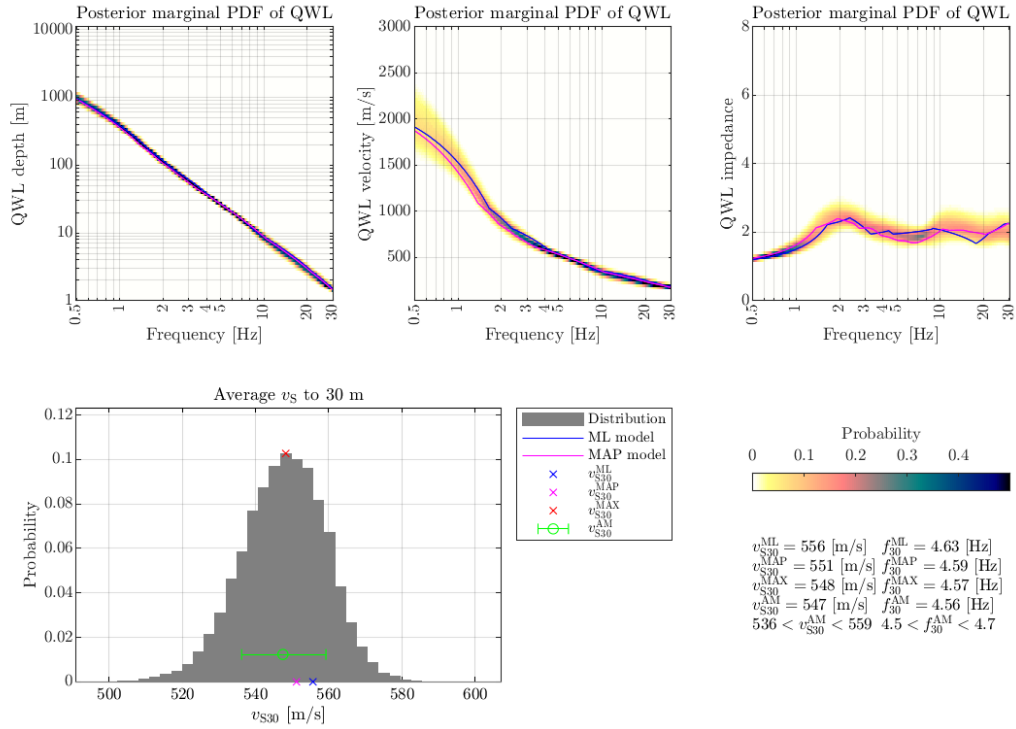
Figure 4: (Top) QWL parameters (depth, velocity, inverse of the impedance contrast; see Poggi et al., 2012) from the inverted Vs profiles. (Bottom) Average Vs30 distribution obtained from the inverted profiles.
