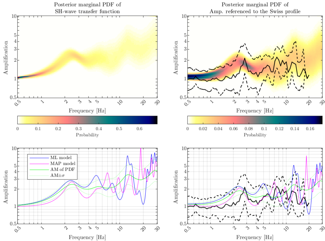
Figure 5: (Top) Posterior marginal PDF on amplification of SH-wave outcrop-surface transfer function in case of unreferenced (left) and referenced (right) to Swiss reference of rock model (Poggi et al., 2011). (Bottom) SH-wave transfer functions for the retrieved ML and MAP models for unreferenced and referenced cases. The black curves represent the EAF from the seismic station and its uncertainty (EAF \pm \sigma ).
