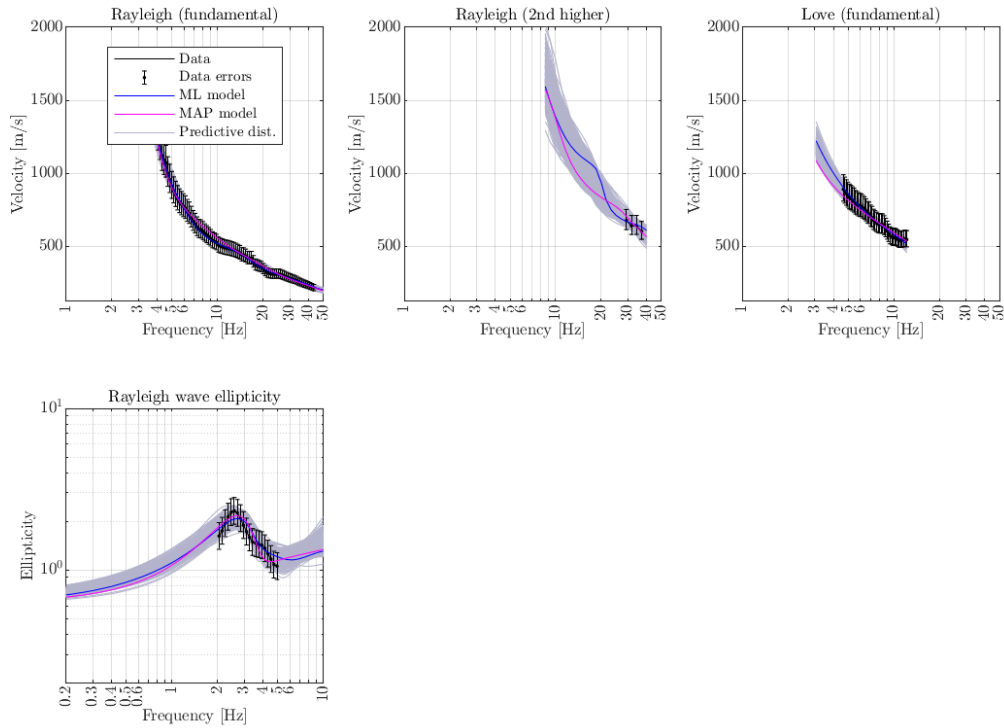
Figure 1: Fit of DCs between the real and modeled data. The real data measured at the site with their uncertainty bounds are shown in black curves with error bars. The modeled data from the inversion are represented as the posterior predictive distribution (grey), ML model (blue), and MAP model (magenta).
