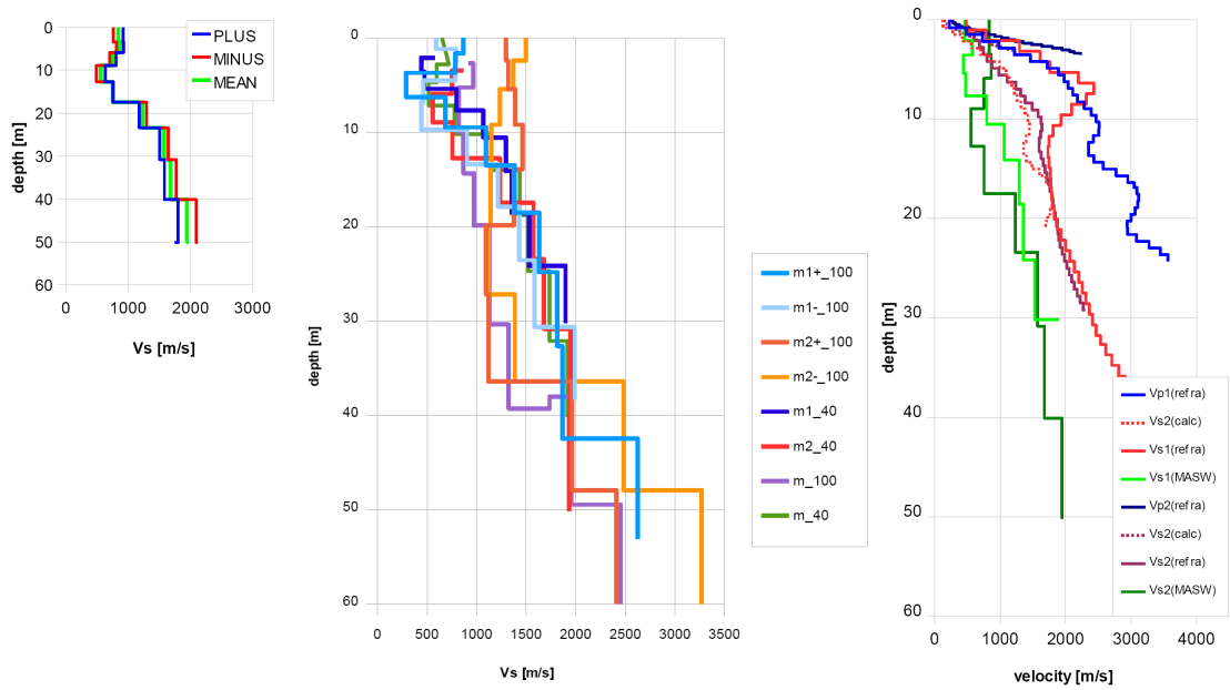
Figure A.2.4. Structural models at site AIGLE without removing structures that do not explain the measured dispersion curves. For more details, see the report of GeoExpert related to the site AIGLE.
